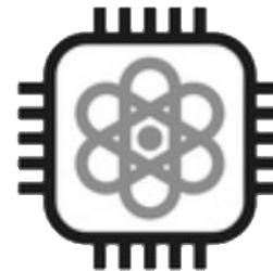
Quantum computing
