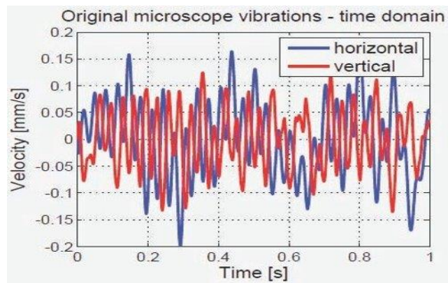
Micro-vibrations before
