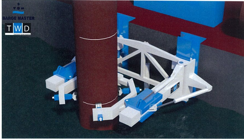
COMPENSATION OF HEAVE, SURGE AND SWAY
